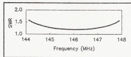
Figure 4—The SWR of the J-pole over the 2-meter band.
